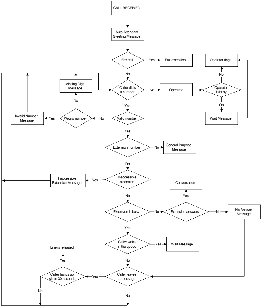
Figure 1- Operation of EVM224 in Day Mode on an Auto Attendant line when Fax Router Mode 1 or Mode 2 is activated as well.
